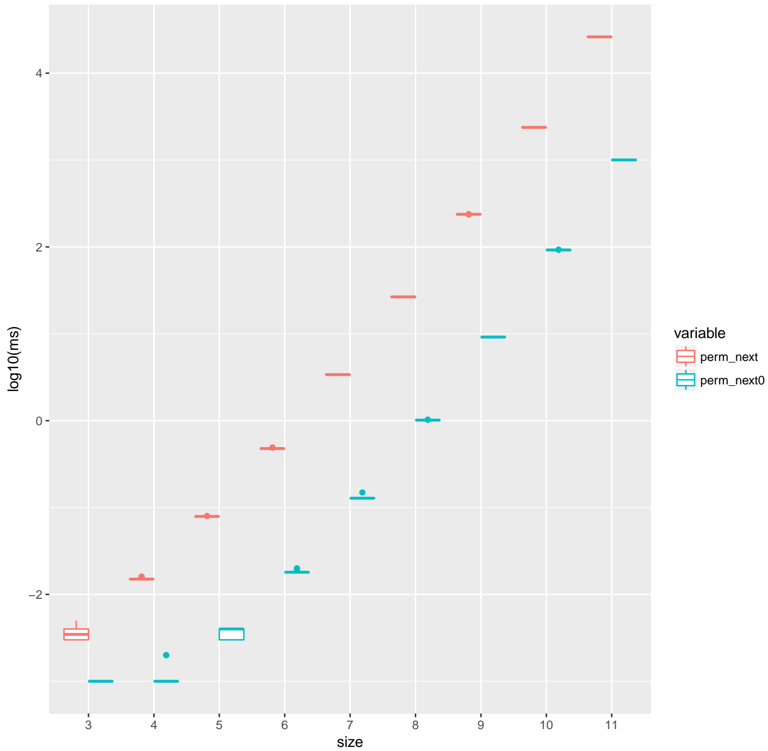
gsl_permutation_next vs gsl_permutation_next0
